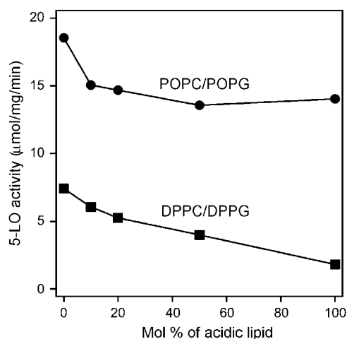
FIGURE 2 Dependence of the specific activity of 5-LO on the content of anionic lipids in fluid (POPC/POPG) and solid (DPPC/DPPG) membranes. Total lipid concentration was 350 \mu\text{M} in all cases, AA concentration was 100 \mu\text{M} , and 5-LO was added to a final concentration of 2.4 \mu\text{g/ml} . The buffer, method of 5-LO activity measurement, and other experimental conditions are described in Materials and Methods.
